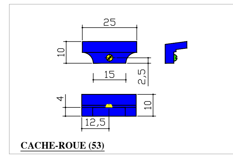
CACHE-ROUE (53)
