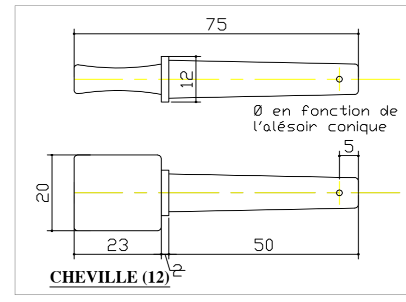
CHEVILLE (12)
